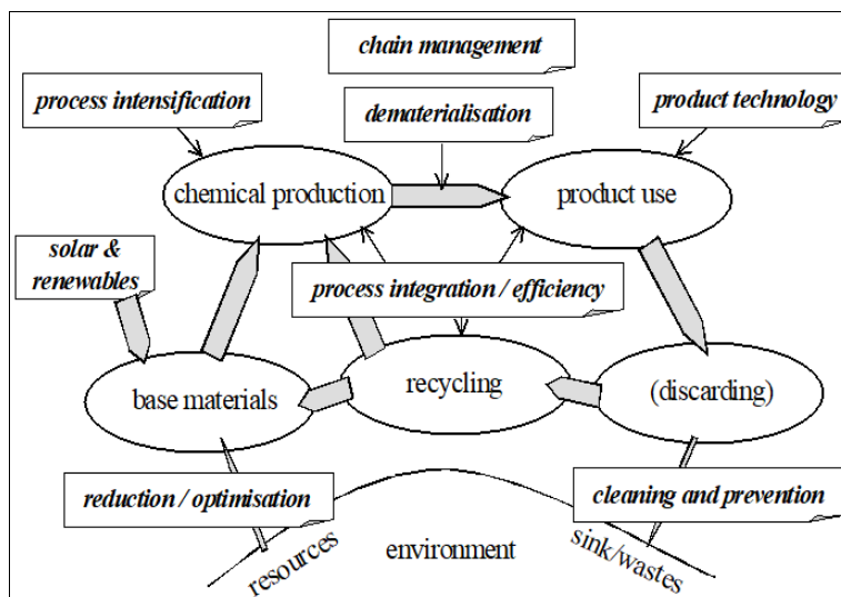
Fig 1: Focal Areas of Chemistry and Chemical Engineering for Sustainable Development [3].
