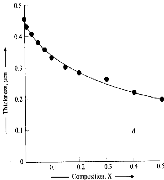
Figure 1d. Variation of thickness with composition parameter, x.
