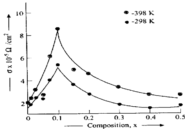
Figure 5. Variation of conductivity with composition parameter, x .
