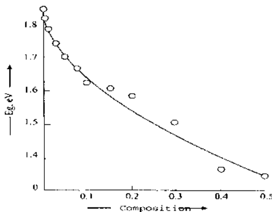
Figure 3. Variation of optical gap, E_g , with composition parameter, x .
