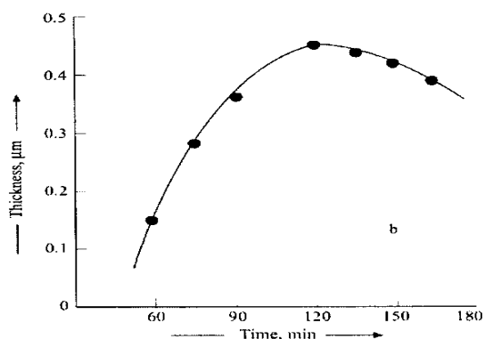
Figure 1b. The terminal thickness versus deposition time at 50 °C.
