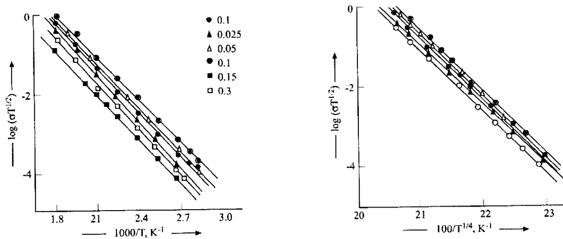
Figure 6b. Variation of \log(\sigma T^{1/2}) versus 100/T^{1/4} for five typical samples.
