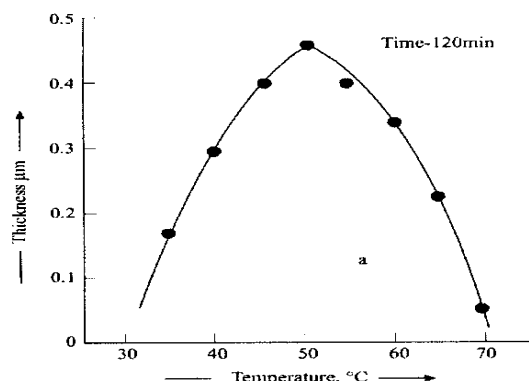
Figure 1a. The terminal thickness versus deposition temperature at 120 minutes.
