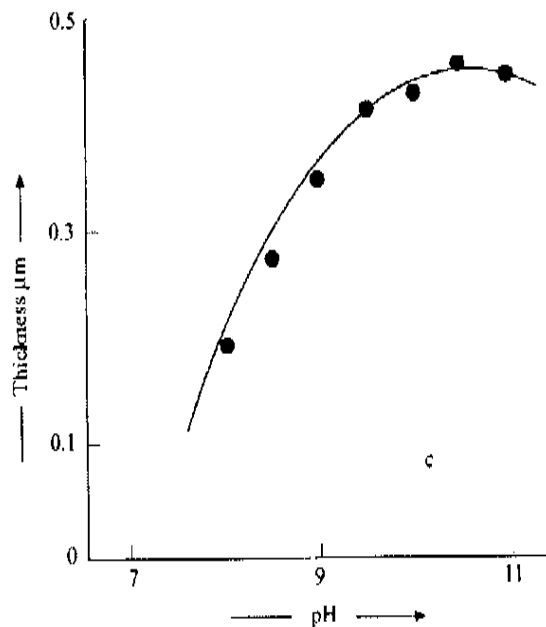
Figure 1c. The terminal thickness versus pH for the above conditions.
