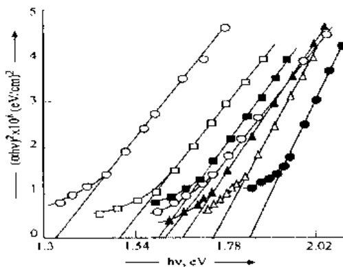
Figure 2. Plot of (\alpha h\nu)^2 versus h\nu for seven typical samples (1) x = 0 (●), (2) x = 0.025 (▲), (3) x = 0.05 (△), (4) x = 0.1 (⊙), (5) x = 0.15 (■), (6) x = 0.3 (□), and (7) x = 0.5 (○)
