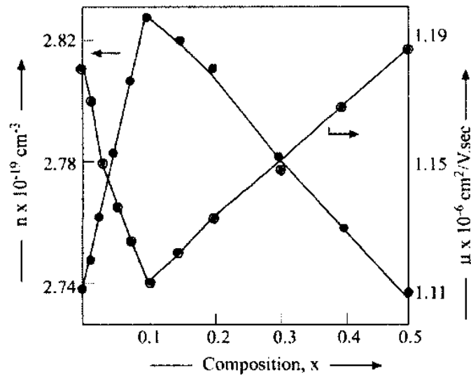
Figure 7. Dependence of carrier density, n , and mobility, \mu , on composition parameter, x .
