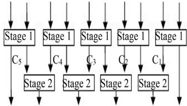
Fig. 2: Signed Digit Addition
