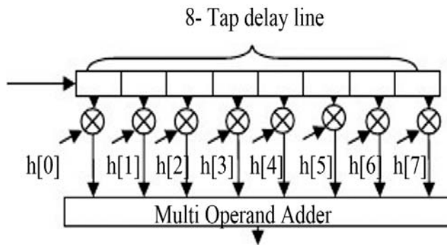
Fig1: Basic FIR Filter
