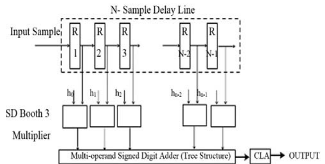
Fig. 4: Signed Digit FIR Filter
