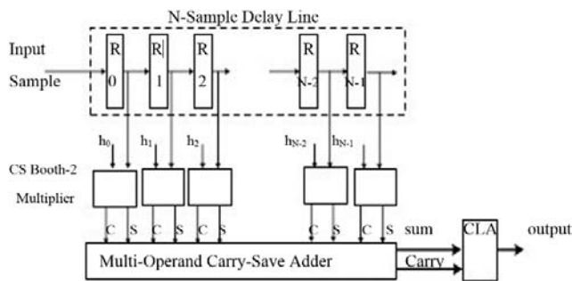
Fig. 5: Carry-Save FIR Filter
