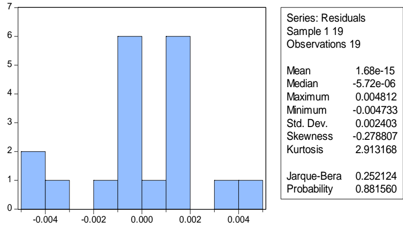
Fig 2: The normality test
