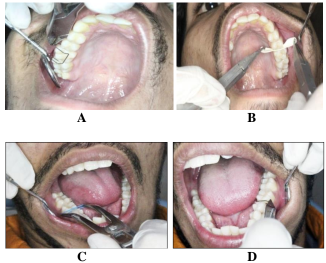
Fig 3: Separators placement: A. Kansal separator in maxillary right side, B. Dumbbell separator in maxillary left side, C. Elastomeric separator in mandibular right side, D. Kesling separator in mandibular left side.
