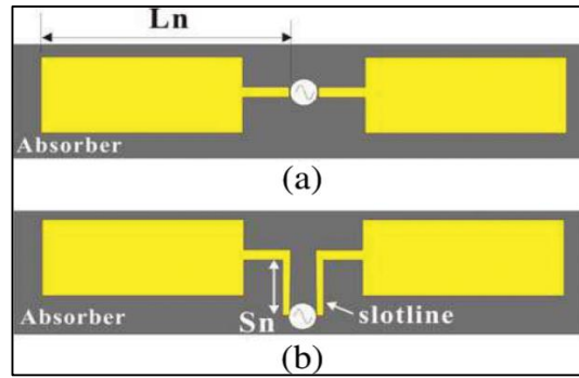
Fig 6: Antenna design process. (a) The 1st stage, (b) the 2 nd stage
