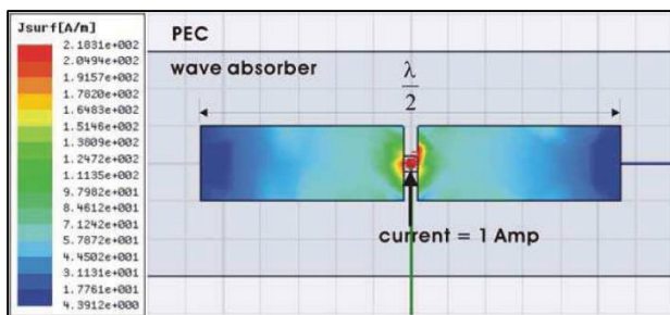
Fig 2: HFSS model of a half-wave dipole
