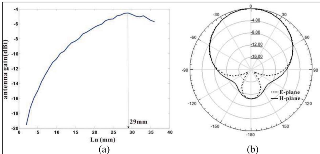
Fig 7: Determination of L_n . (a) Antenna gain variation by sweeping L_n , (b) radiation pattern of L_n = 26 mm
