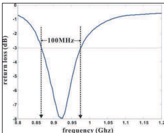
Fig 10: Measured impedance bandwidth of the metal tag
