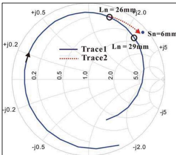
Fig 8: Impedance matching process using Smith Chart
