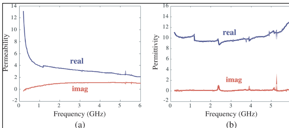
Fig 4: Measured material constants of CIP wave absorber. (a) Permeability, (b) Permittivity
