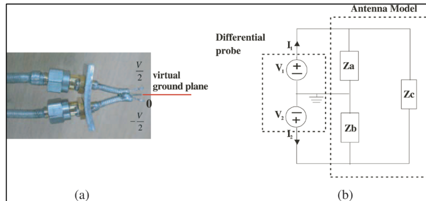
Fig 9: Adjusting the antenna impedance using the differential probe. (a) Differential probe, (b) the antenna is considered as a two-port network
