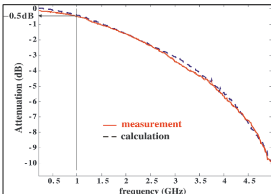
Fig 5: Attenuation of magnetic composite material made by carbonyl iron powder
