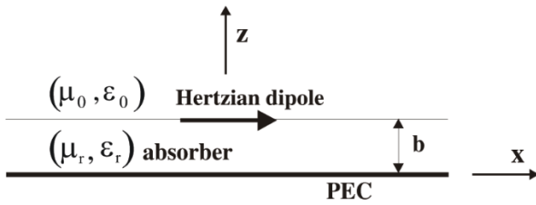
Fig 1: A Hertzian dipole on a grounded magnetic composite material
