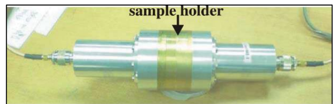
Fig 3: Measurement of material constants using coaxial probe system
