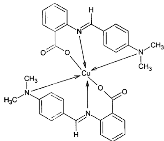
Structure of the complex [CuL_2]
