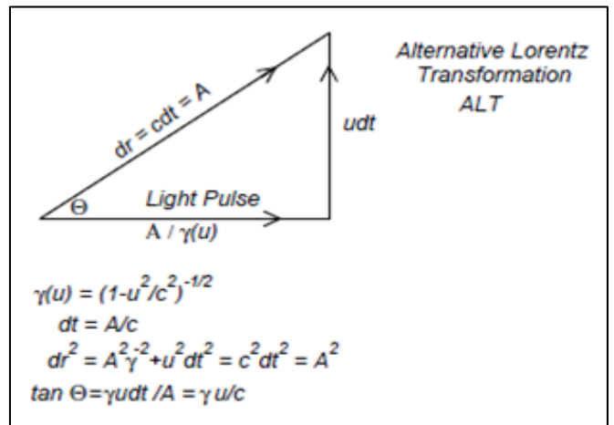
Fig 2: Diagram showing a light pulse traveling in a transverse direction on a satellite that is moving with speed u relative to observer O. The distance dr = A traveled by the light pulse is computed from O's vantage point by employing the alternative Lorentz transformation (ALT) discussed in the text [8,9]. He finds that the light pulse travels at an angle \Theta = \tan^{-1} (\gamma u / c) and with speed equal to c , so that his measured elapsed time is dt = A/c . Another observer (M) at rest on the satellite, who agrees to use the same unit of time as O, i.e. the same clock rate, also finds the light pulse to travel the same distance from his perspective ( dr' = A ) at the same speed c , but in a different direction ( \Theta = 0 ). The elapsed time for this event measured by M is therefore dt' = A/c , the same value as for O. The light pulse therefore arrives at the same time at its detector on the satellite for the two observers, despite the fact that they are in relative motion to each other.
