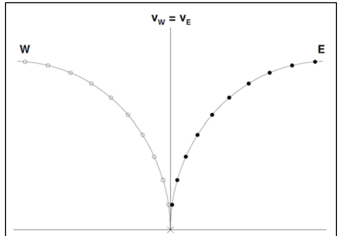
Fig 1: Diagram showing two rockets leaving the same position in a gravity-free region of space. Their speed relative to the departure position is the same for both at all times, even though the respective directions of velocity are always different. The symmetric relationship of their trajectories indicates that the rates of their respective onboard clocks are always the same. This remains true even for the termini of the trajectories shown, in which case the rockets are both a) inertial systems (each traveling at constant velocity) and b) in relative motion to one another at that point.
