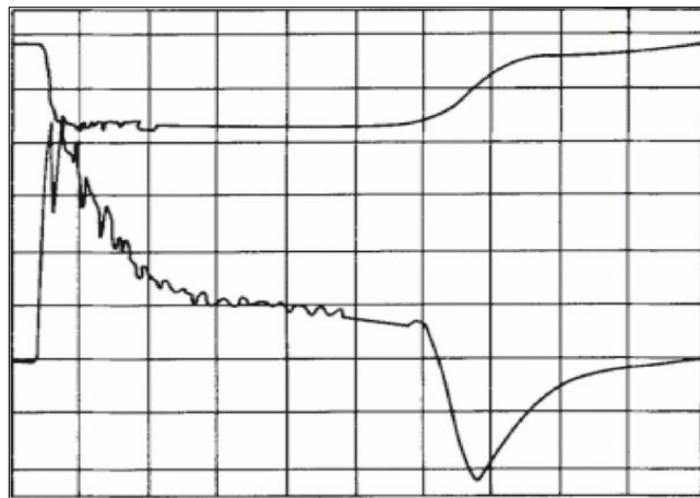
Fig 3: A Typical oscilloscope trace for the applied bias (Top) and the corresponding current through current transformer (bias). Top trace has y-axis 2000v/div and x-axis 500 ns/div. bottom trace has y-axis 100ma/div and x-axis ns/div. plasma density 6.26 \times 10^8 per cc. note the current behaviour in the flat top of the applied bias. The model predicts the current in this portion
