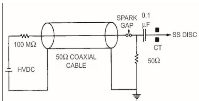
Fig 2: Pulse Forming Network, CT is the Pearson Current Transformer
