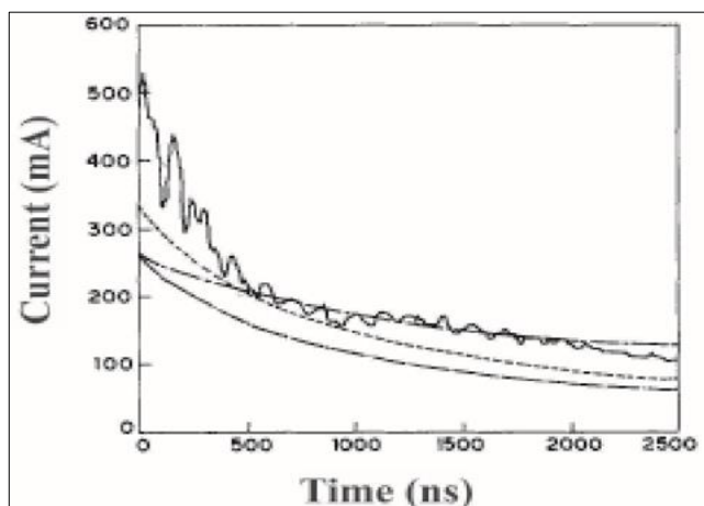
Fig 4: Comparison between the Current Obtained in (i) Experiment (—) (ii) the Model [Eq. (7)] (----) (iii) Conduction Current [Eq. (2)] (.....) (iv) Model [Eq. (7)] and Contribution from the Emitted Secondary Electrons (— · — · —). Applied Bias is 3010V and Plasma Density is 9.4 \times 10^8 /cc.
