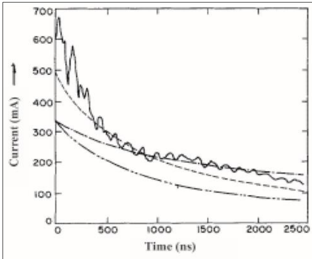
Fig 5: Comparison Between the Current Obtained in (i) Experiment (---) (ii) the Model [Eq. (7)] (----) (iii) Conduction Current Eq. (2) (-.-.-) (iv) Model [Eq. (7)] and Contribution from the Emitted Secondary Electrons (.....). Applied Bias is 4900 V and Plasma Density is 9.4 \times 10^8/cc
